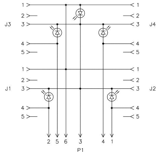
WIRING DIAGRAM
